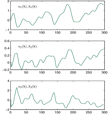
Figure 1. System states x_k and their estimates \hat{x}_k
