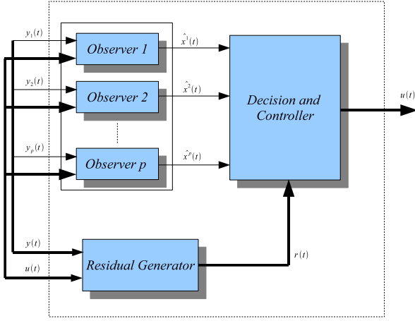
Fig. 1. Fault detection and fault tolerant control block
